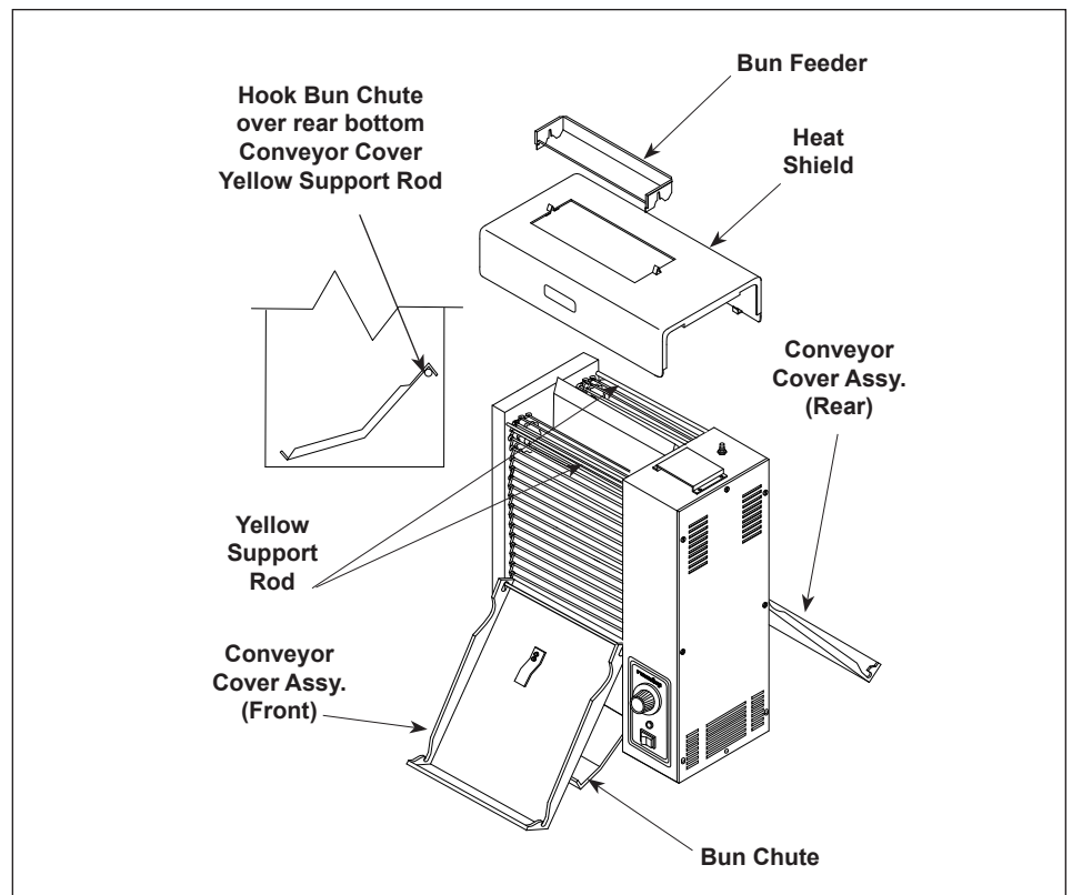
Figure 2. Installing Bun Chute
