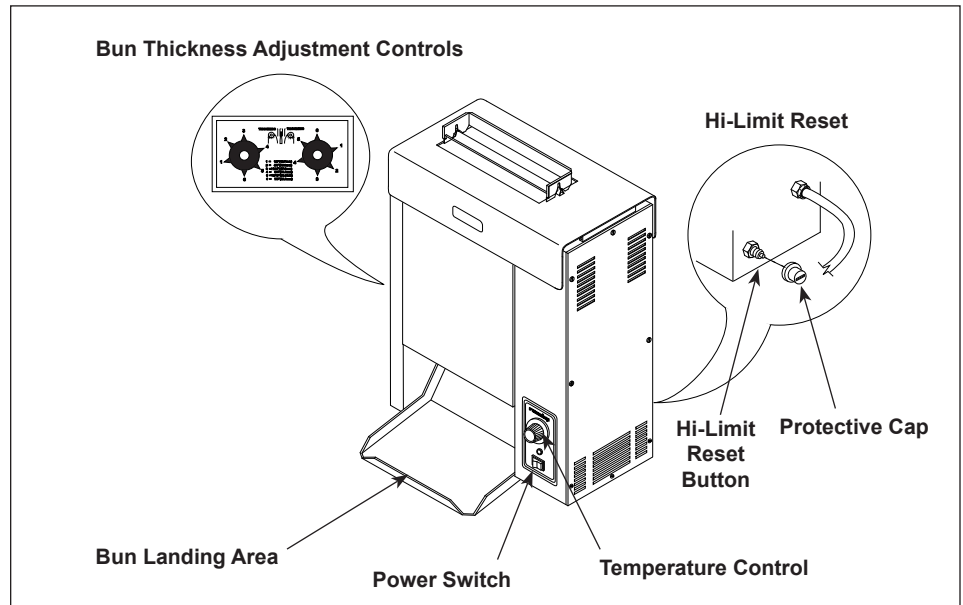
Figure 3. Toaster Controls
