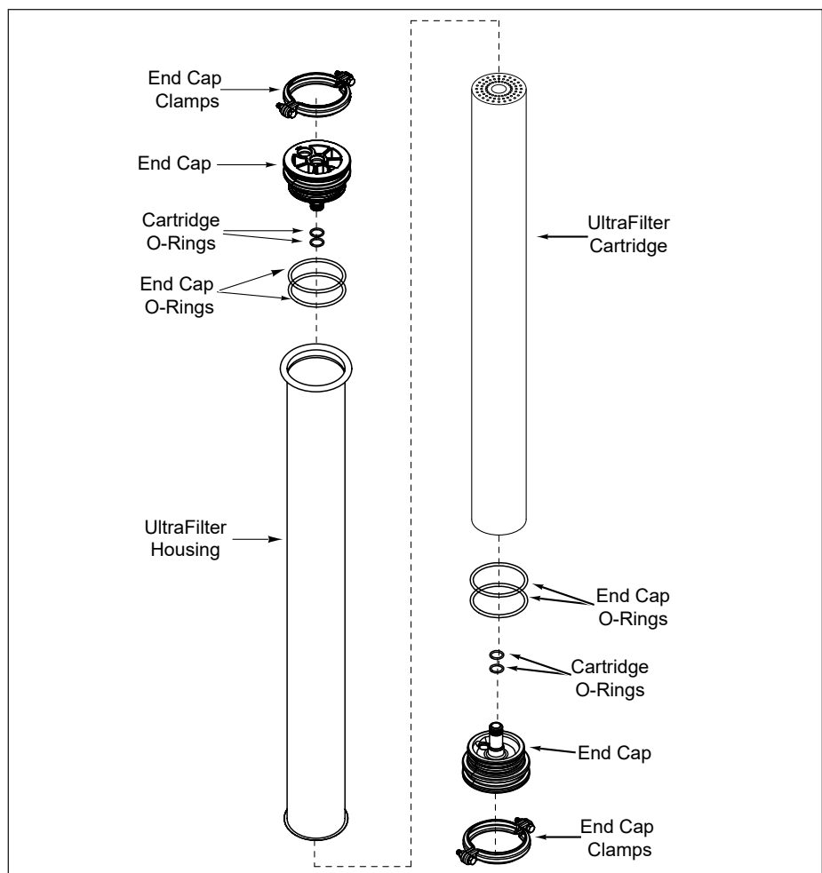
Figure 9. Replacing the Ultra Filter Cartridge
