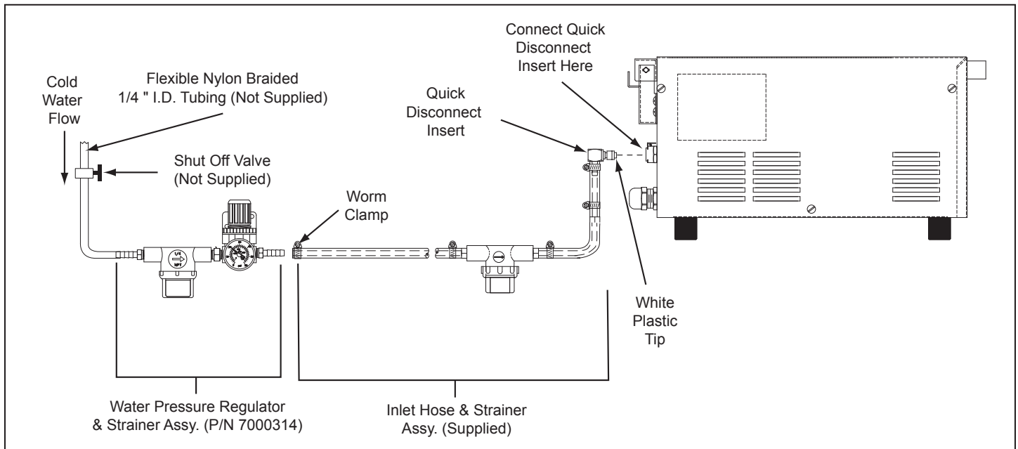
Figure 2. Connecting Water Supply to DFW-250
