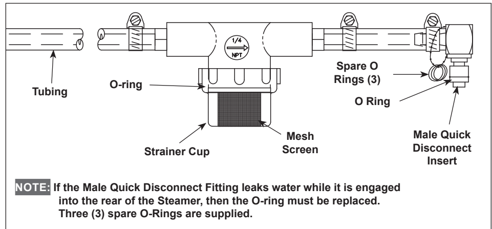
Figure 7. Inlet Hose Assembly
