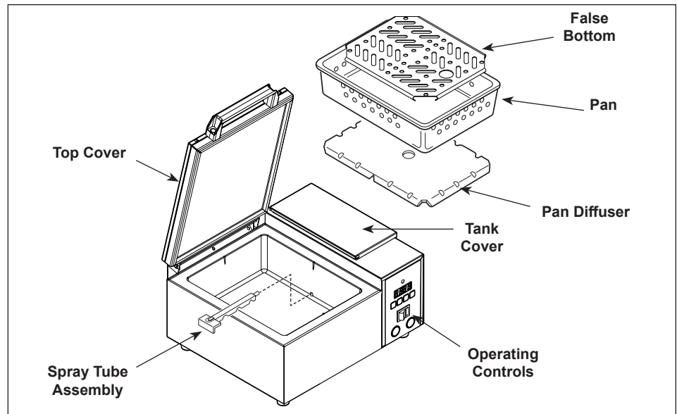
Figure 1. Components
