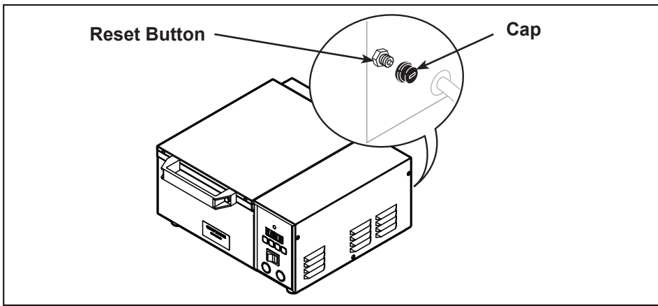
Figure 4. Hi-Limit Reset Button
