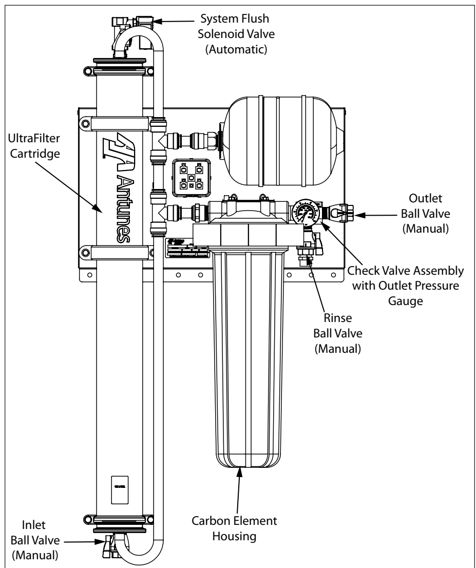
Figure 1. System Components
