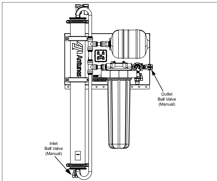
Figure 6. Inlet and Outlet Connections
