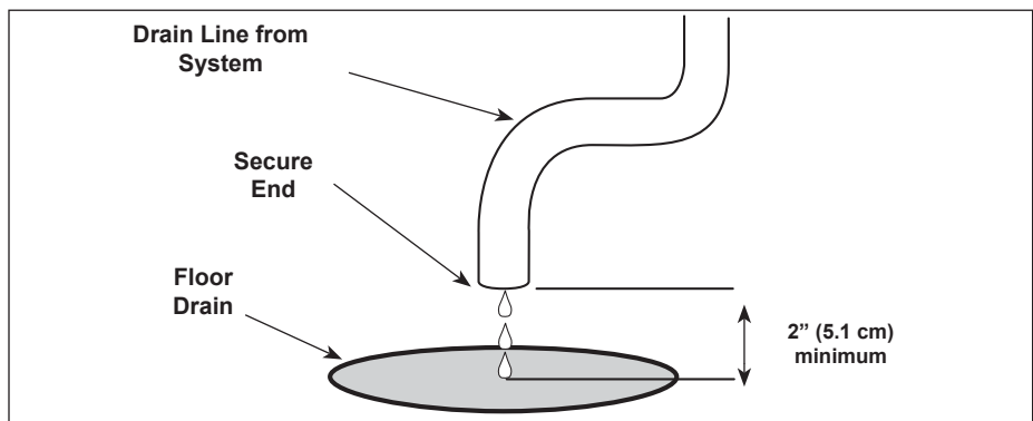
Figure 4. Drain Line Plumbing
