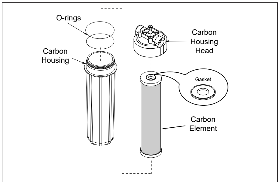
Figure 9. Carbon Element
