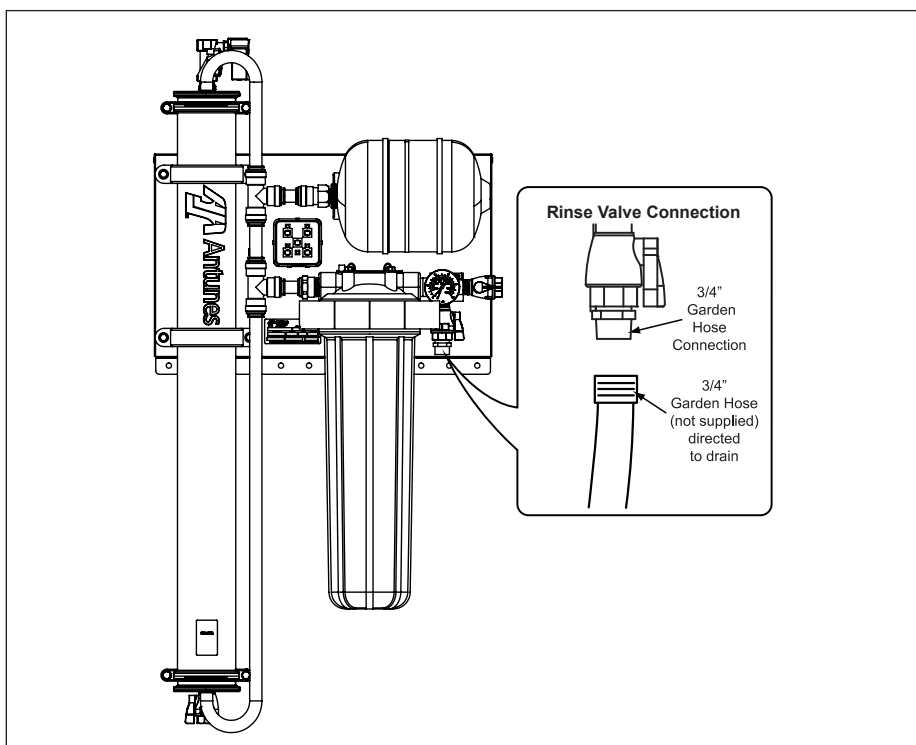
Figure 5. Rinse Valve Connection
