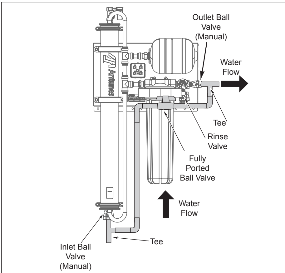
Figure 7. Install Bypass
